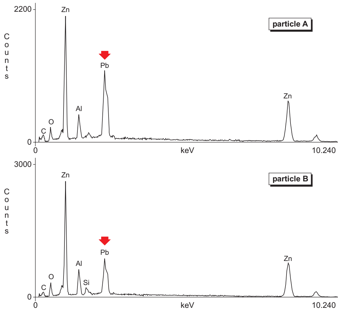
Fig. 9 Corrosion products largely filling a crack and lead particles along crack paths (two analysed by EDX)
