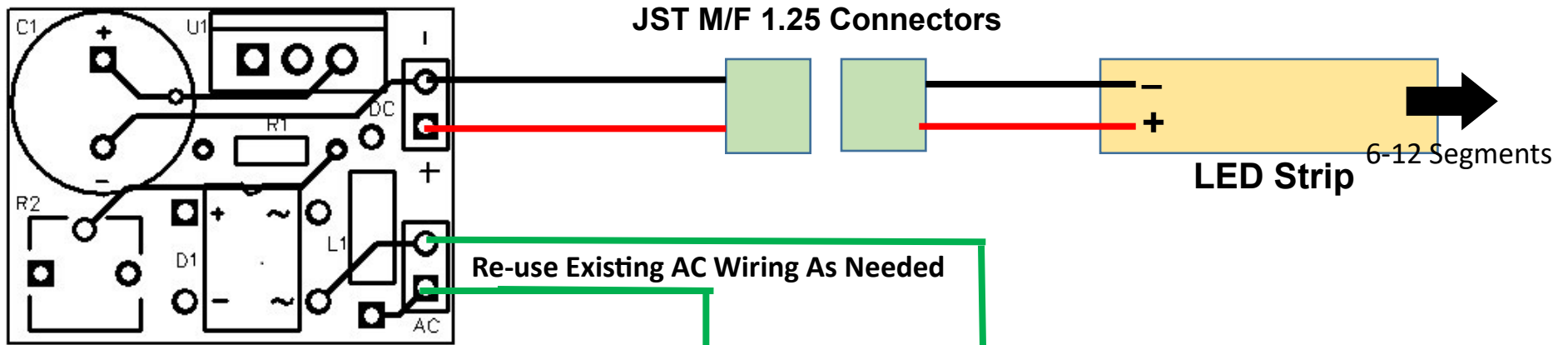
Lighting Module
