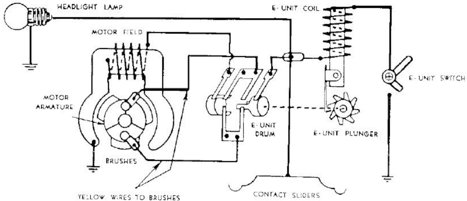
Figure 2 - Schematic Wiring Diagram of a Typical E-Unit Installation
