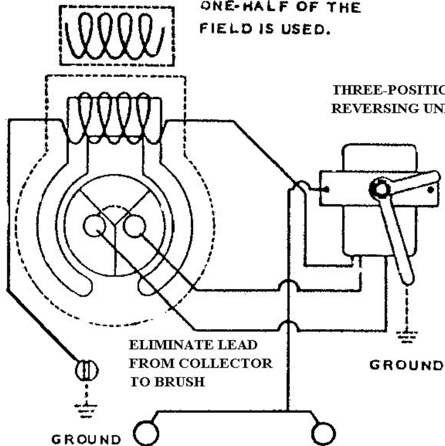
MOTOR CONVERTED TO THREE-POSITION REVERSE
