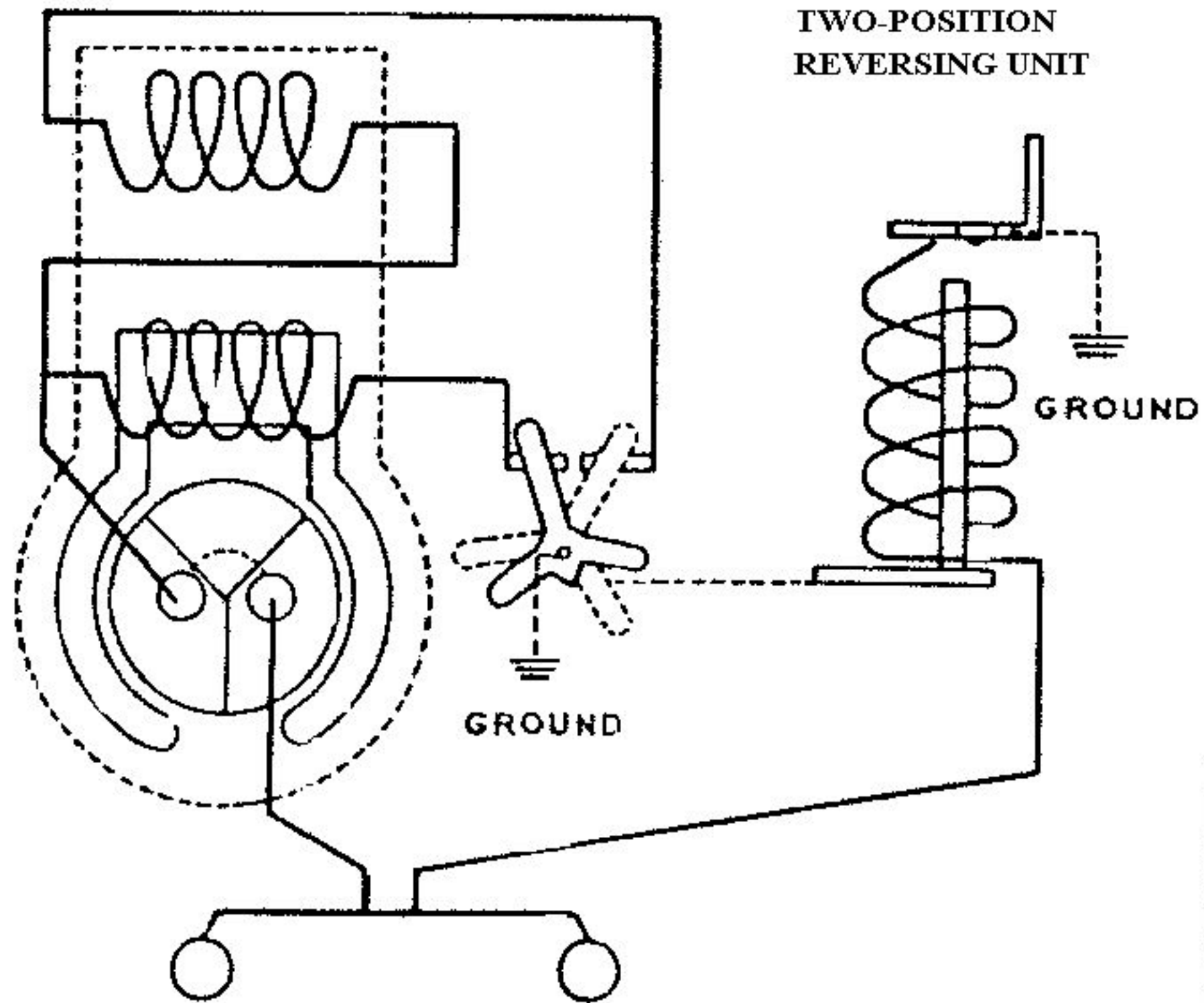
MOTOR USING A TWO-POSITION REVERSE
