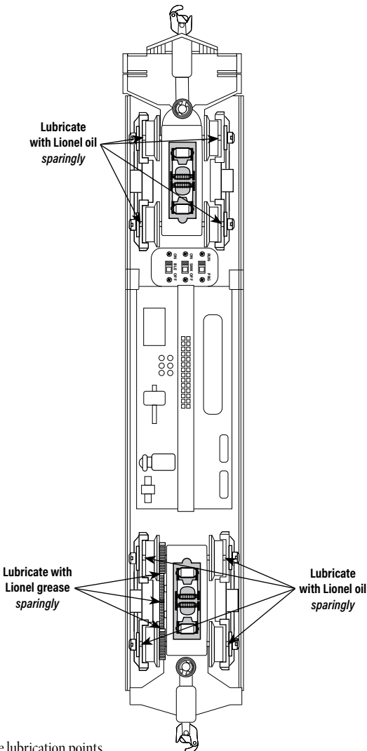
Figure 16. Locomotive lubrication points
