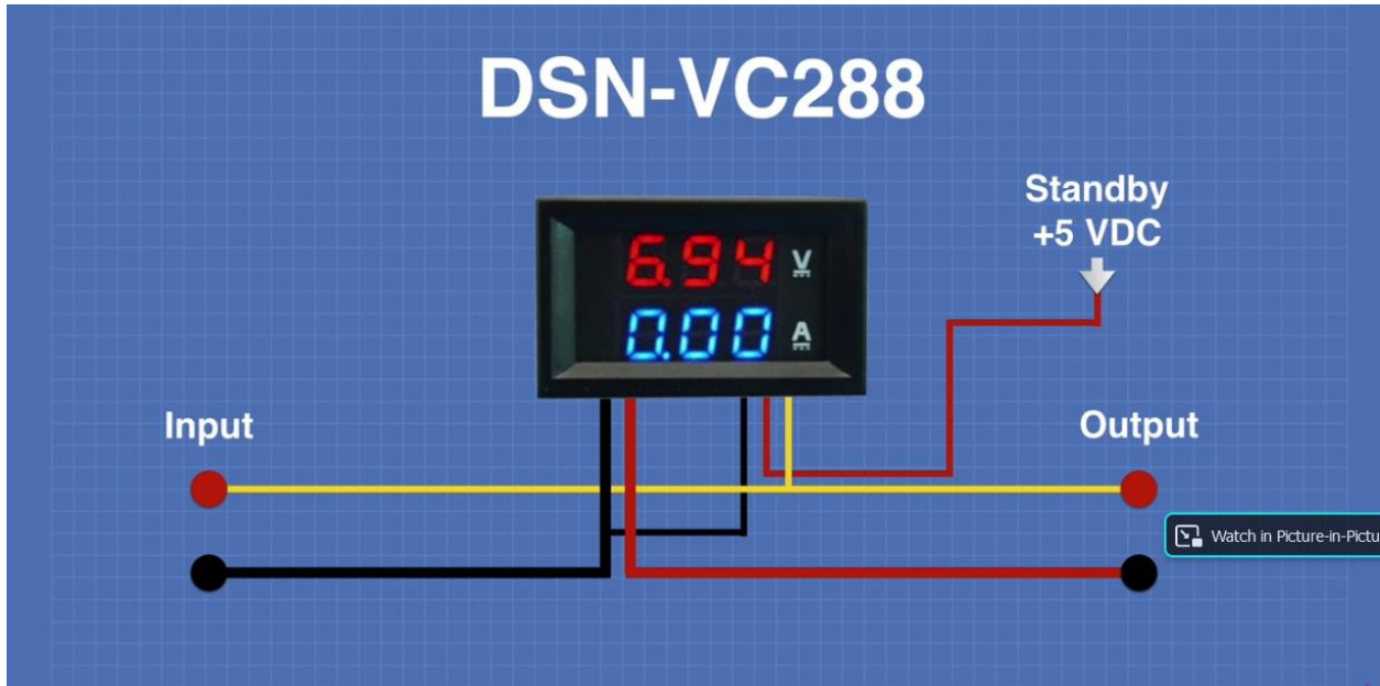
Image from You Tube Video: ATX Bench Power Supply - Convert a Computer Power Supply https://www.youtube.com/watch?v=n_A-jkpijcm
