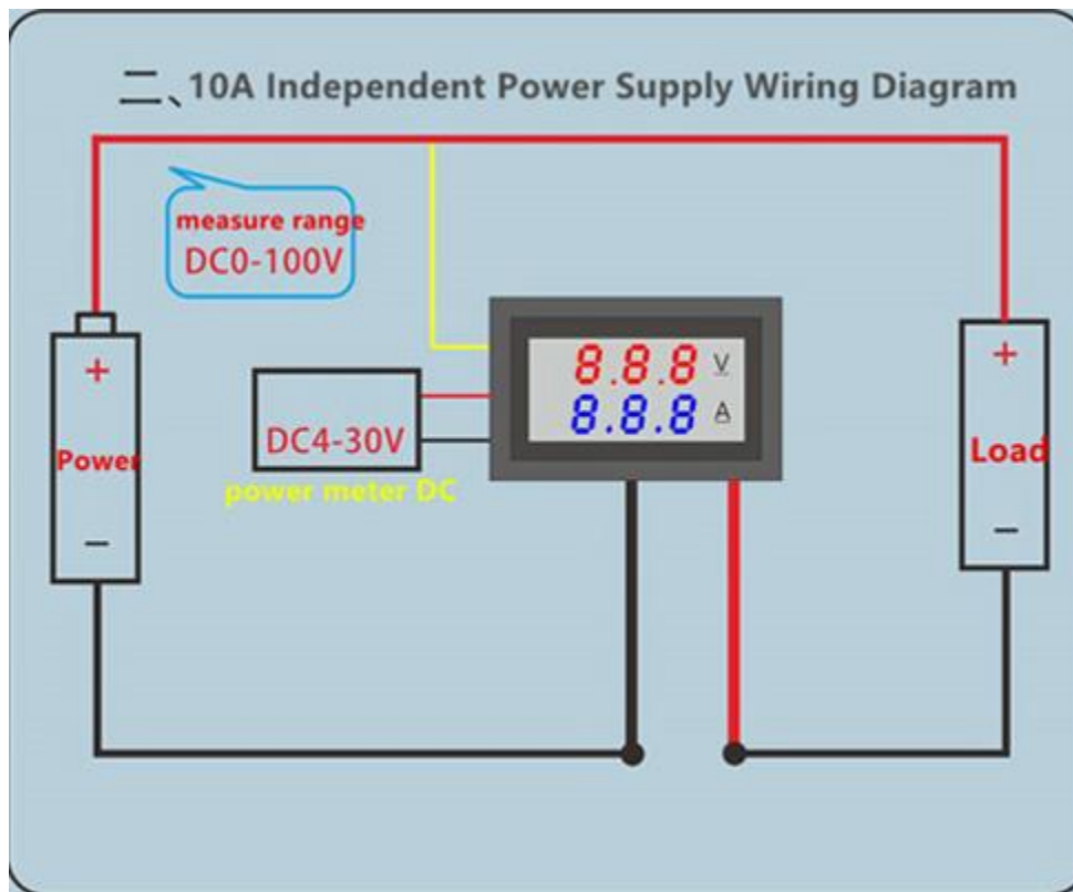
Image from diymore Digital Voltmeter Ammeter instructions on Amazon ... https://www.amazon.com/dp/B08HQM1RMF?psc=1&ref=ppx_yo2_dt_b_product_details
