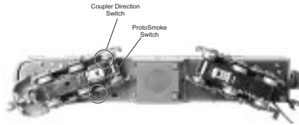
Figure 1: Locating The Smoke Unit & ProtoCoupler Selection Switch
