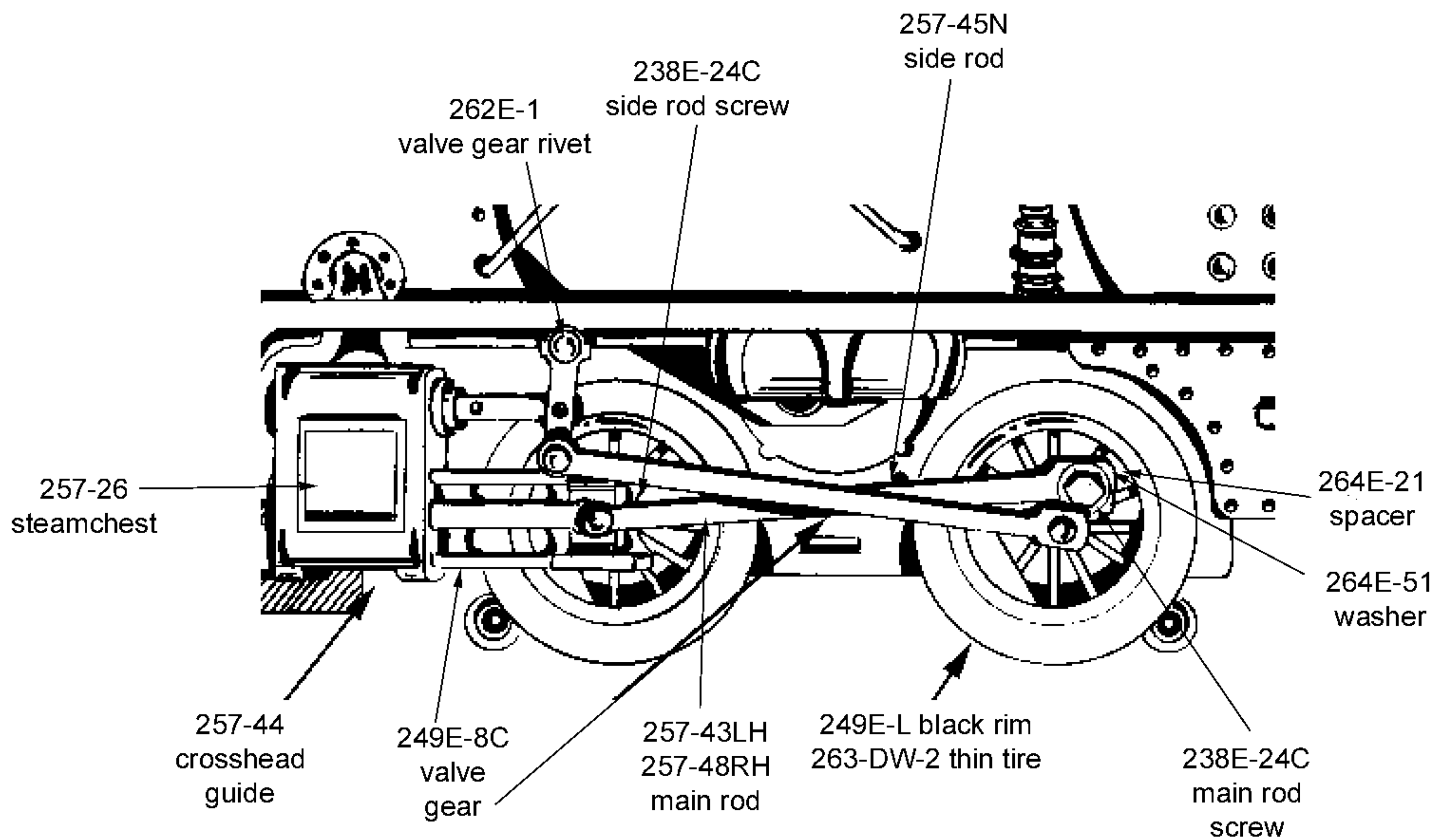
249 LINK PAC complete set of all rods, spacers, screws, rivets for loco linkage
