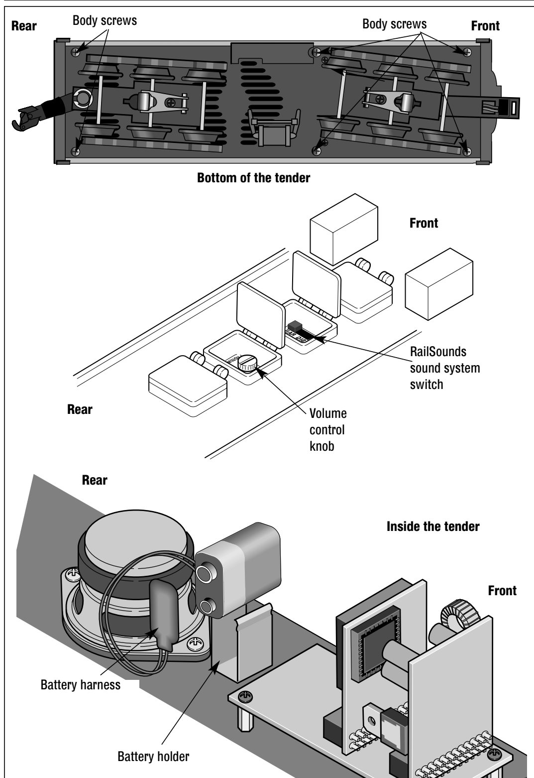
Figure 4. RailSounds sound system controls and battery installation
