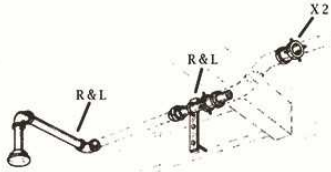
PSH-4391 Water line connection & coupling cored for .060" wire w/mounting bracket, tender or engine, R&L, 2 ea.
