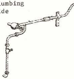
PSH-40159 Super-heater plumbing fireman's side, Challenger
