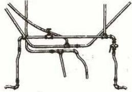
PSDR-1171 Hi-pressure lubrication lines, used w/4123 & 4442, K-36, 37 & some 27's & 28's
