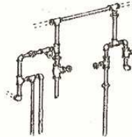
PSSH-8554 Tee-boiler backhead auxiliary piping PSSH-8554-1 Plastic
