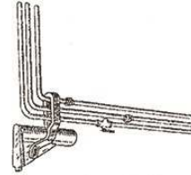
PSK-40136 Challenger air plumbing & damper control for power reverse
