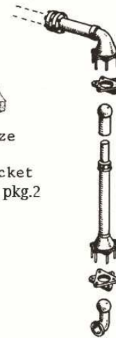
PSH-4458 Steam supply fittings w/working ball joint, for booster engine, set
