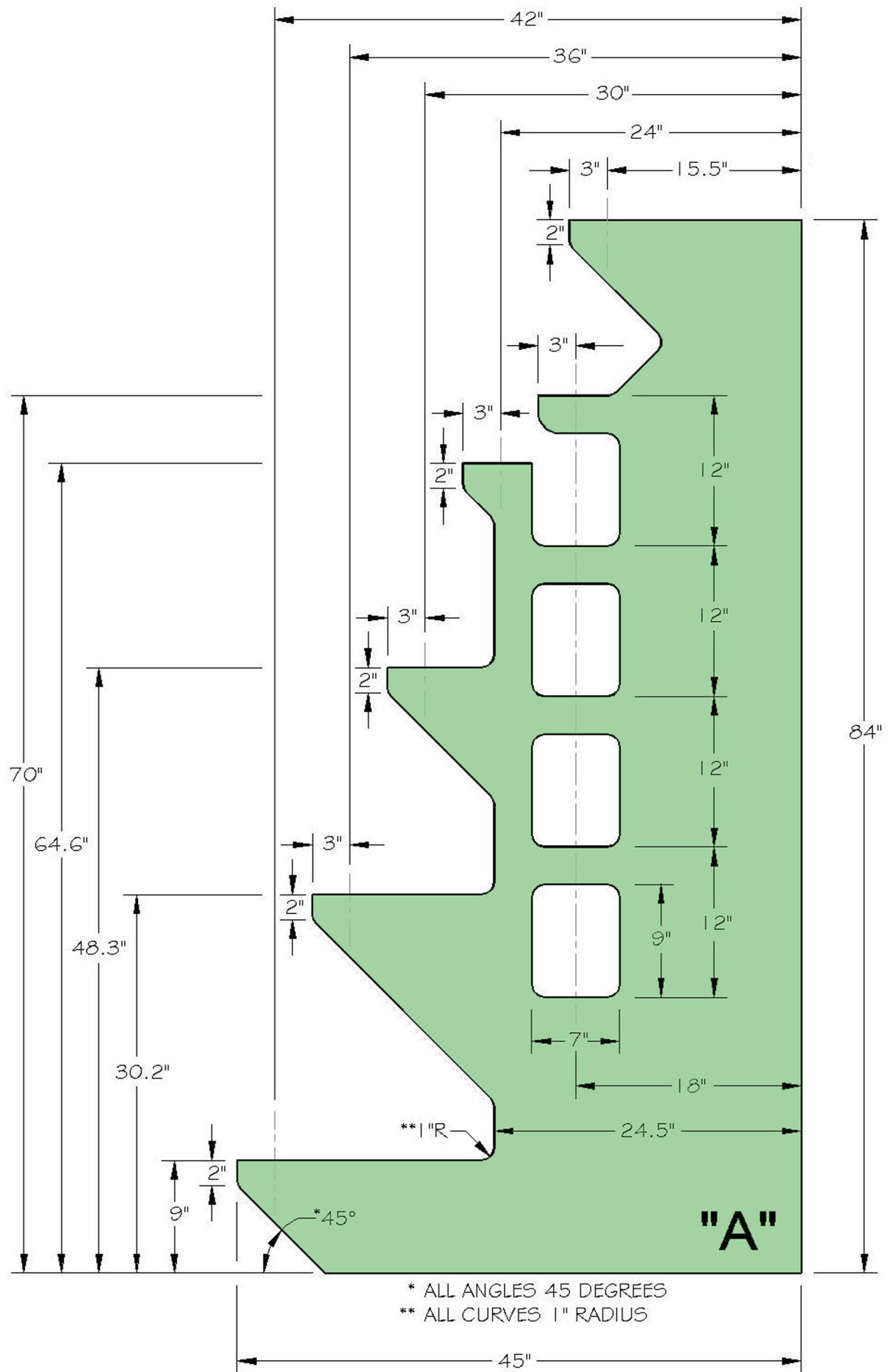
VERTICAL SECTION "A" PLAN
