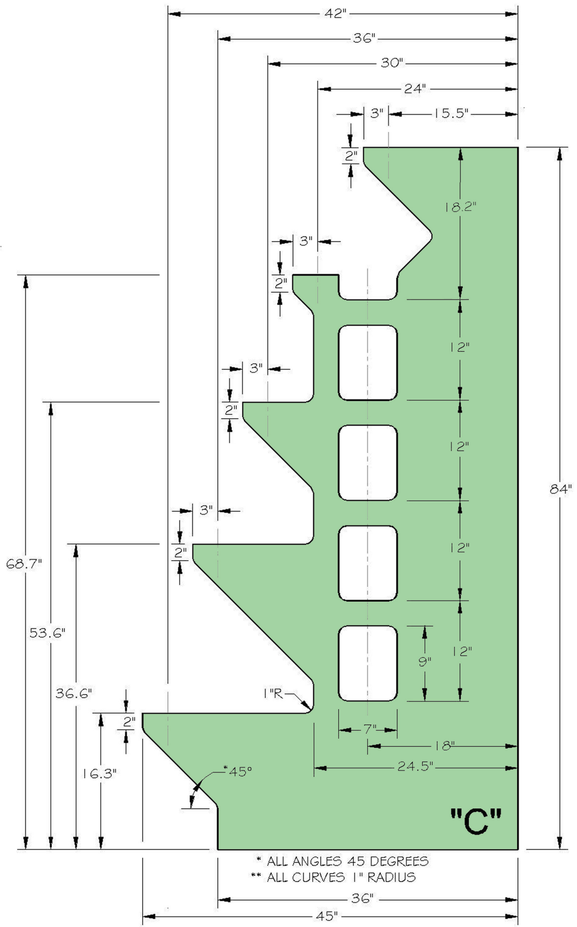
VERTICAL SECTION "C" PLAN
