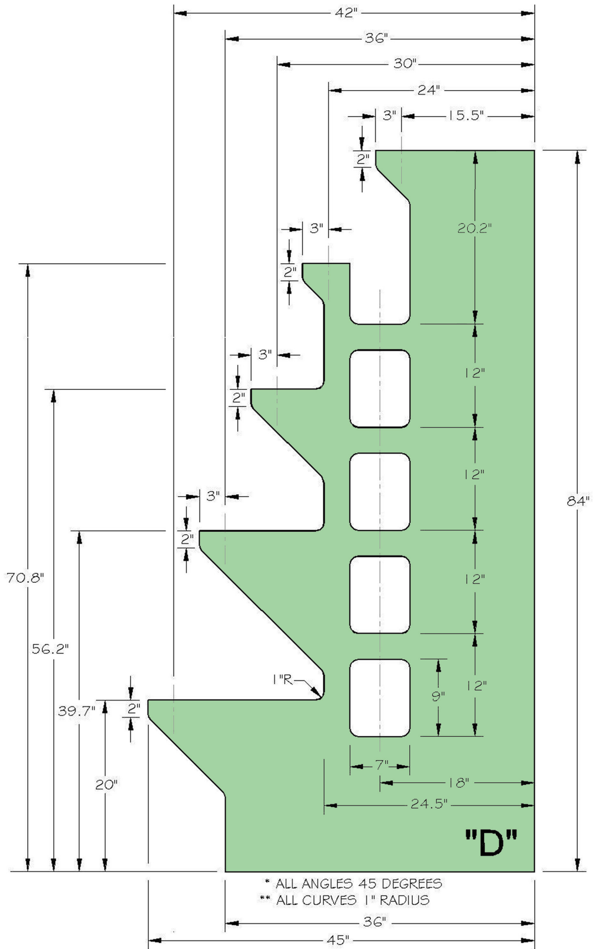
VERTICAL SECTION "D" PLAN
