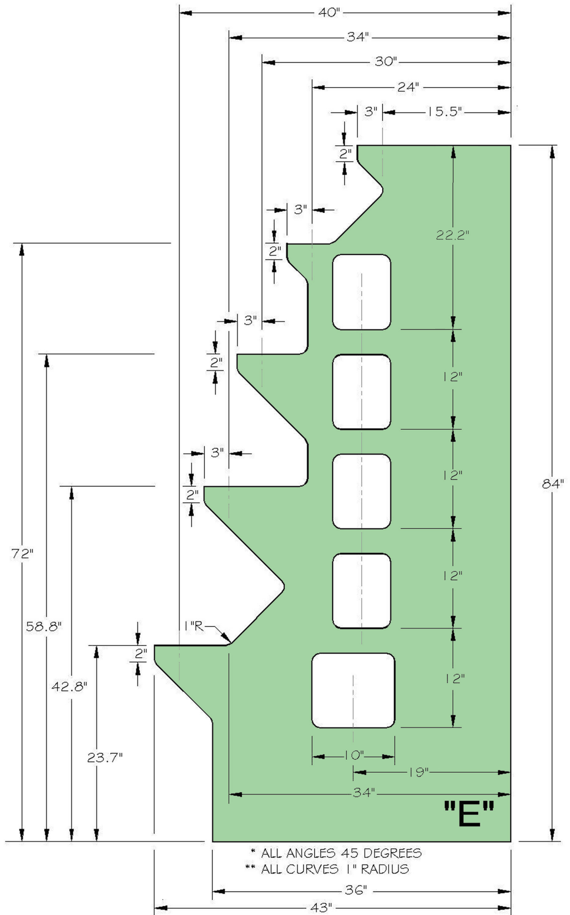
VERTICAL SECTION "E" PLAN
