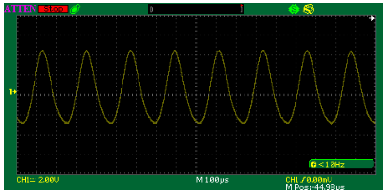
Figure 3 .005µF Capacitive Load (2V/div)
