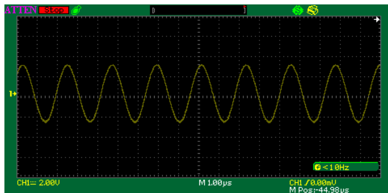
Figure 2 .001µF Capacitive Load (2V/div)
