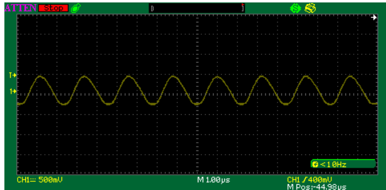
Figure 6 .047uf Capacitive Load (500mv/div)
