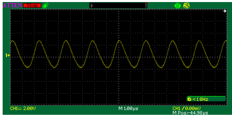
Figure 4 .01uf Capacitive Load (2V/div)
