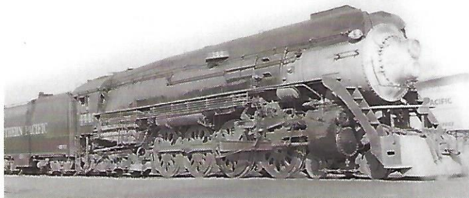
Version 3 GS-4 4430~4447 with skirts removed and large lettering on the tenders
