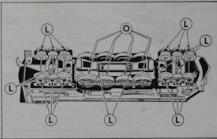
Lubricating Points of Lionel No. 662 Locomotive in which the Motor is Mounted Lengthwise
