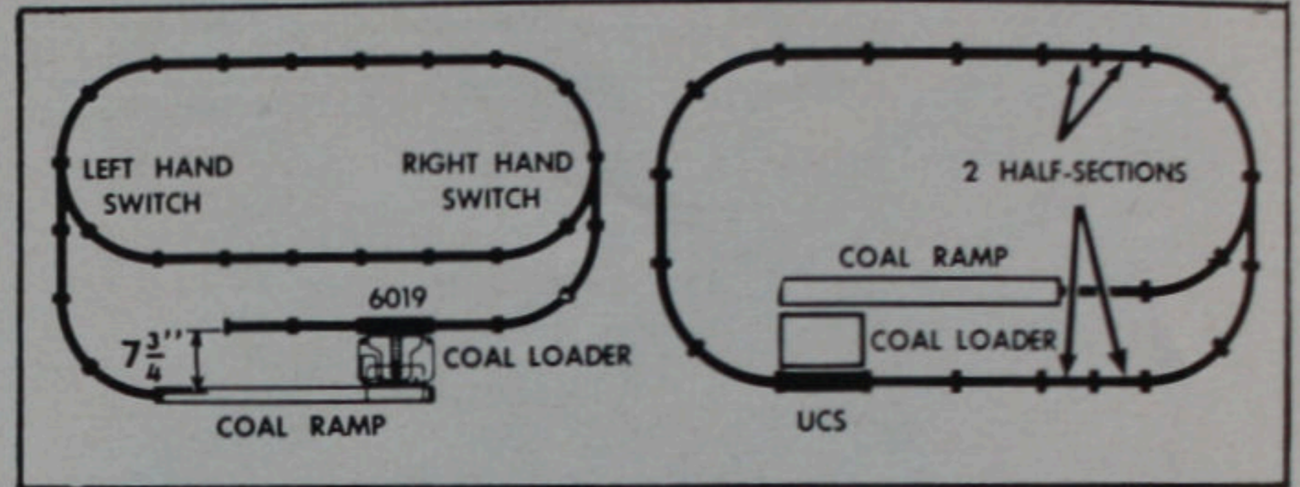
Typical Layouts for Combined Operation of 456 Coal Ramp and 397 Coal Loader: "027" on the Left, "O" on the Right.
