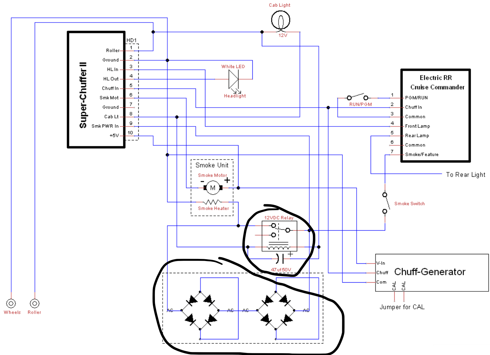
Figure 2: Typical Installation with ERR Cruise Commander, Idle Smoke Intensity, and Chuff-Generator
